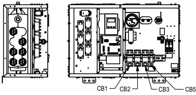
SINGLE PHASE 6-ELEMENT BOILER (1P6E)
