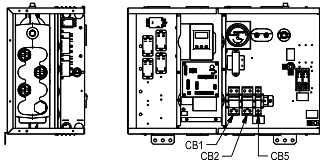
SINGLE PHASE 3-ELEMENT BOILER (1P3E)
