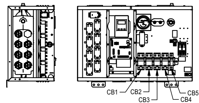
SINGLE PHASE 7-ELEMENT BOILER (1P7E)
