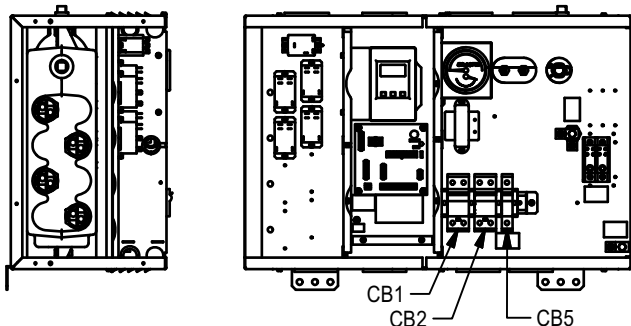
SINGLE PHASE 4-ELEMENT BOILER (1P4E)
