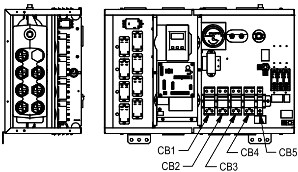
3 PHASE 7-ELEMENT BOILER (3P7E)
