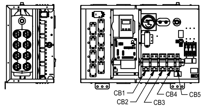
3 PHASE 8-ELEMENT BOILER (3P8E)
