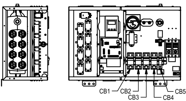
SINGLE PHASE 8-ELEMENT BOILER (1P8E)
