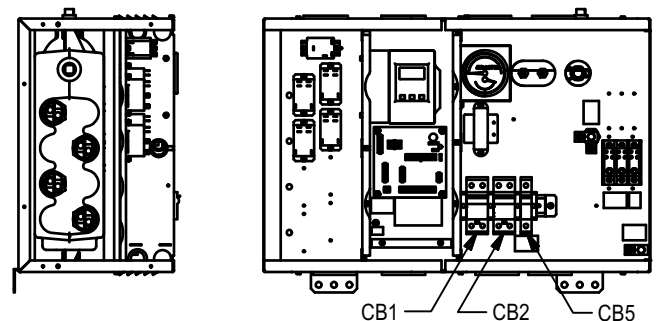
3 PHASE 4-ELEMENT BOILER (3P4E)
